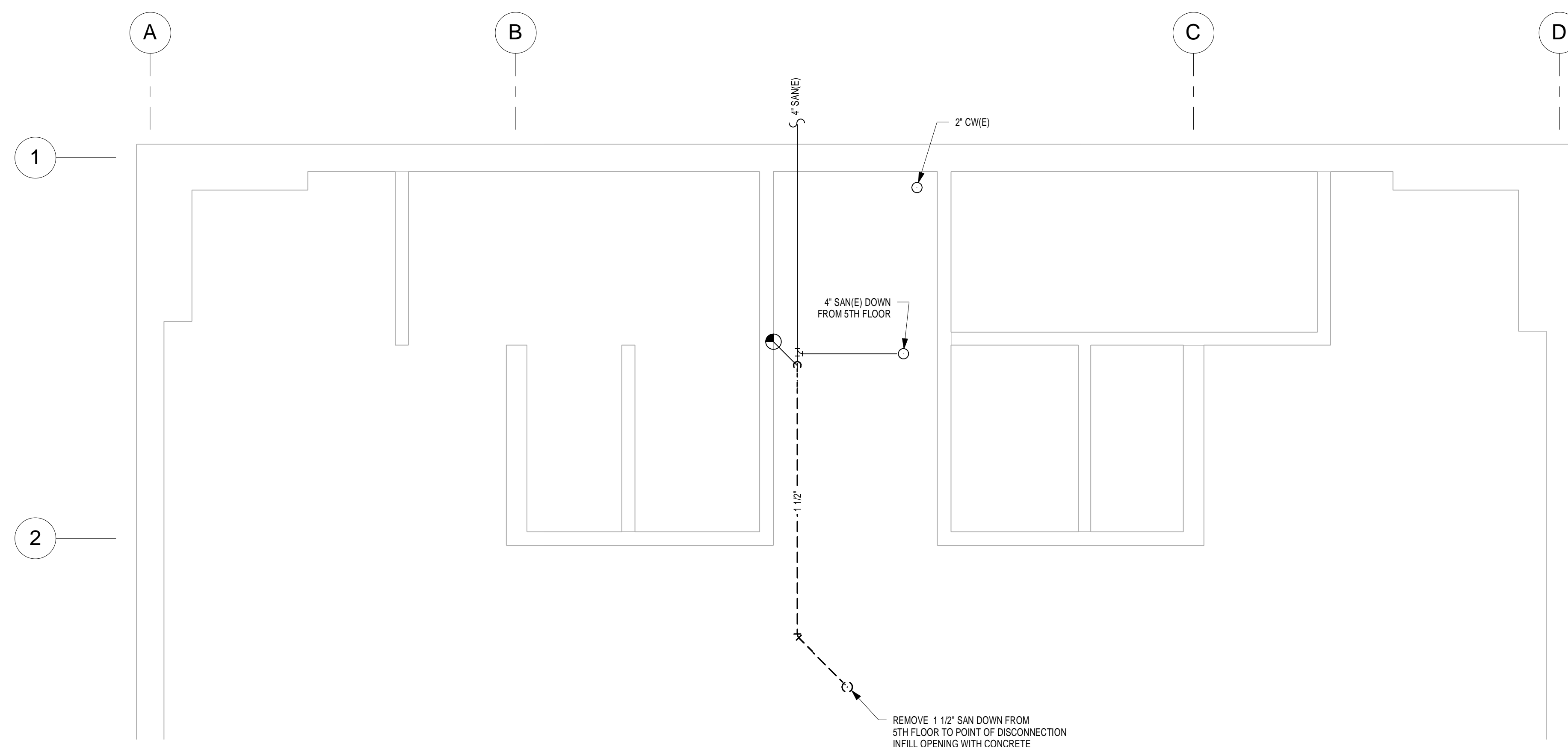
② 4TH FLOOR PLUMBING - DEMO 1/4" = 1'-0"
