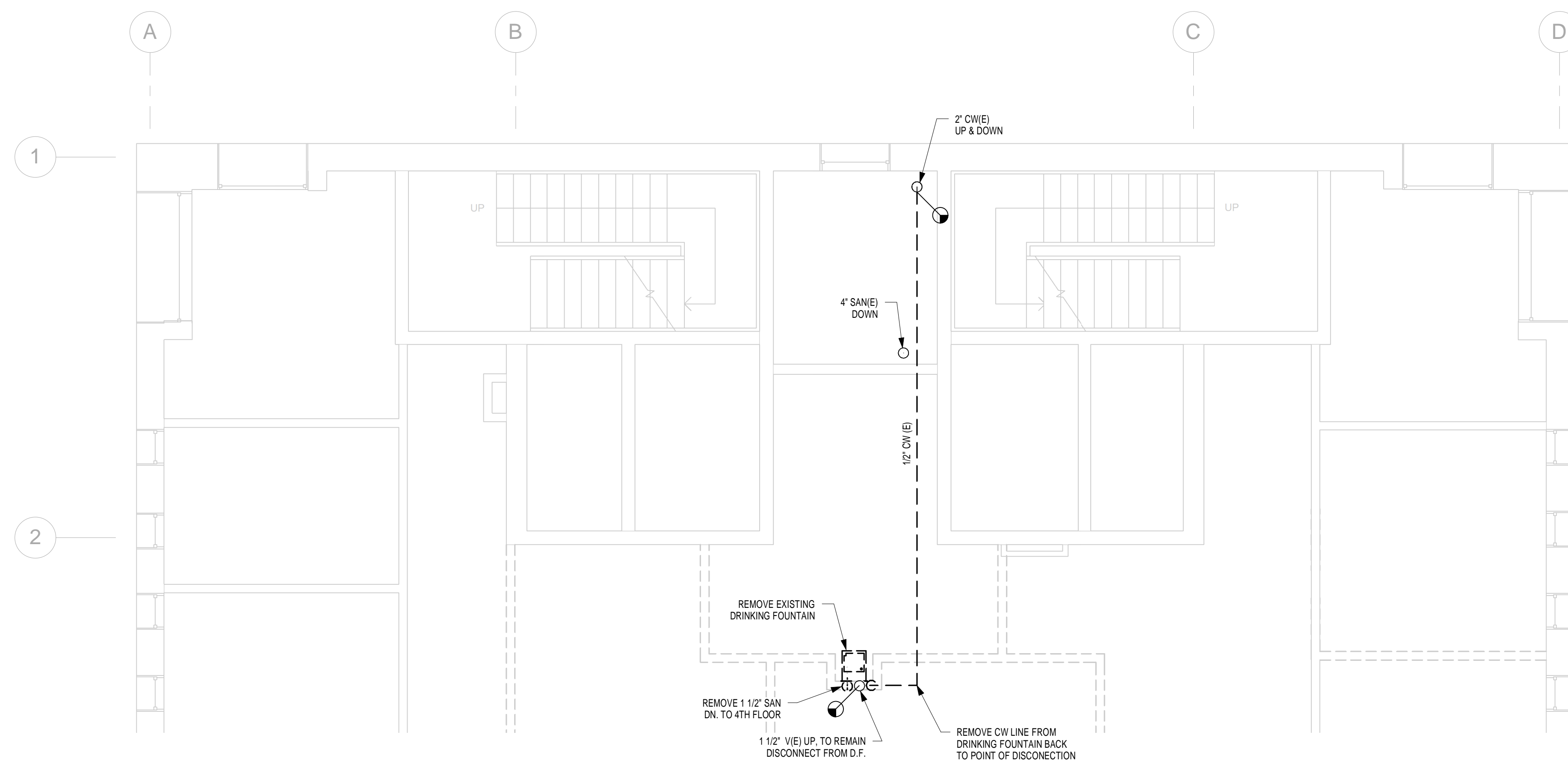
① 5TH FLOOR PLUMBING - DEMO 1/4" = 1'-0"
