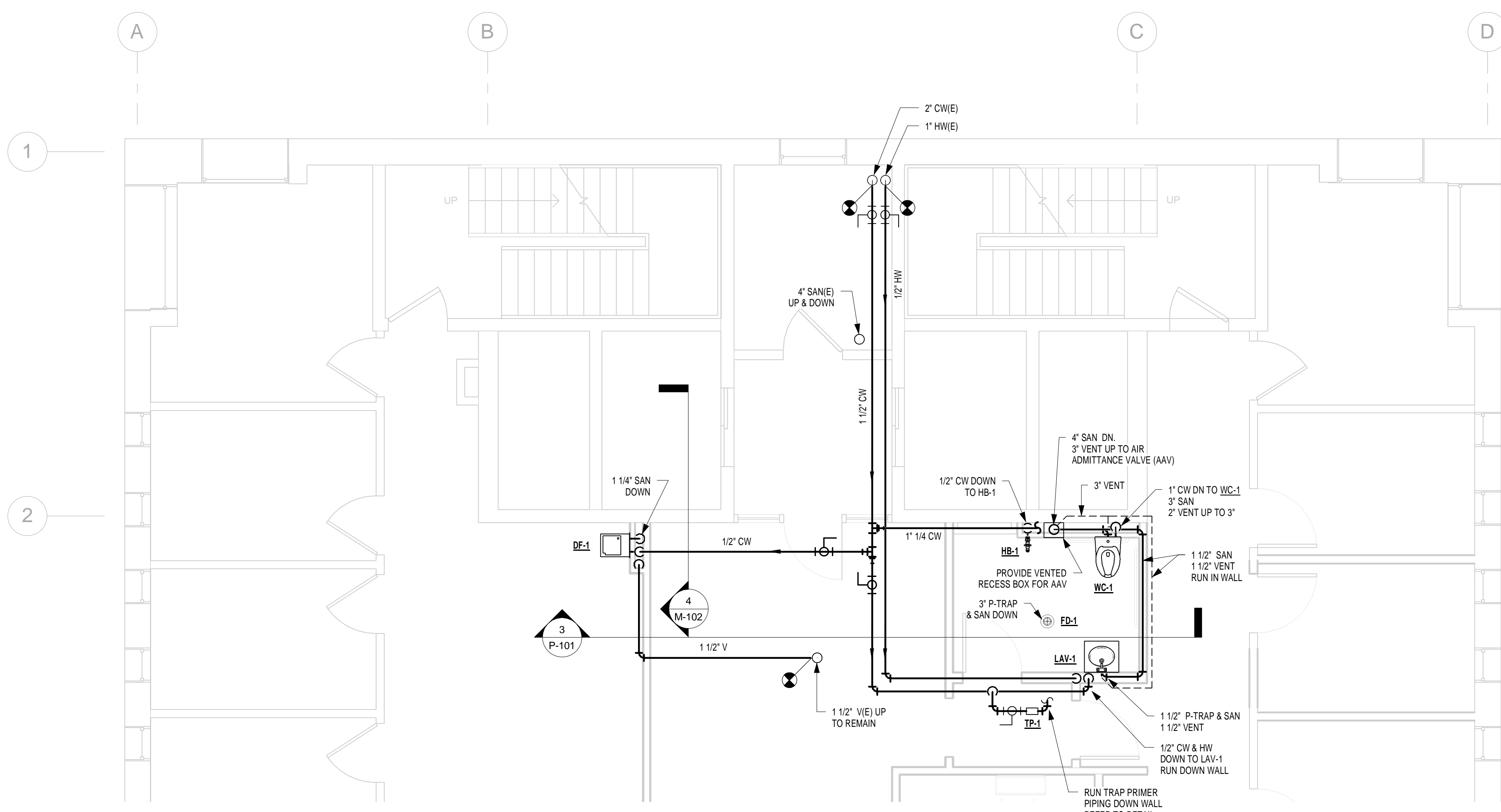
1 5TH FLOOR PLUMBING PLAN 1/4" = 1'-0"
