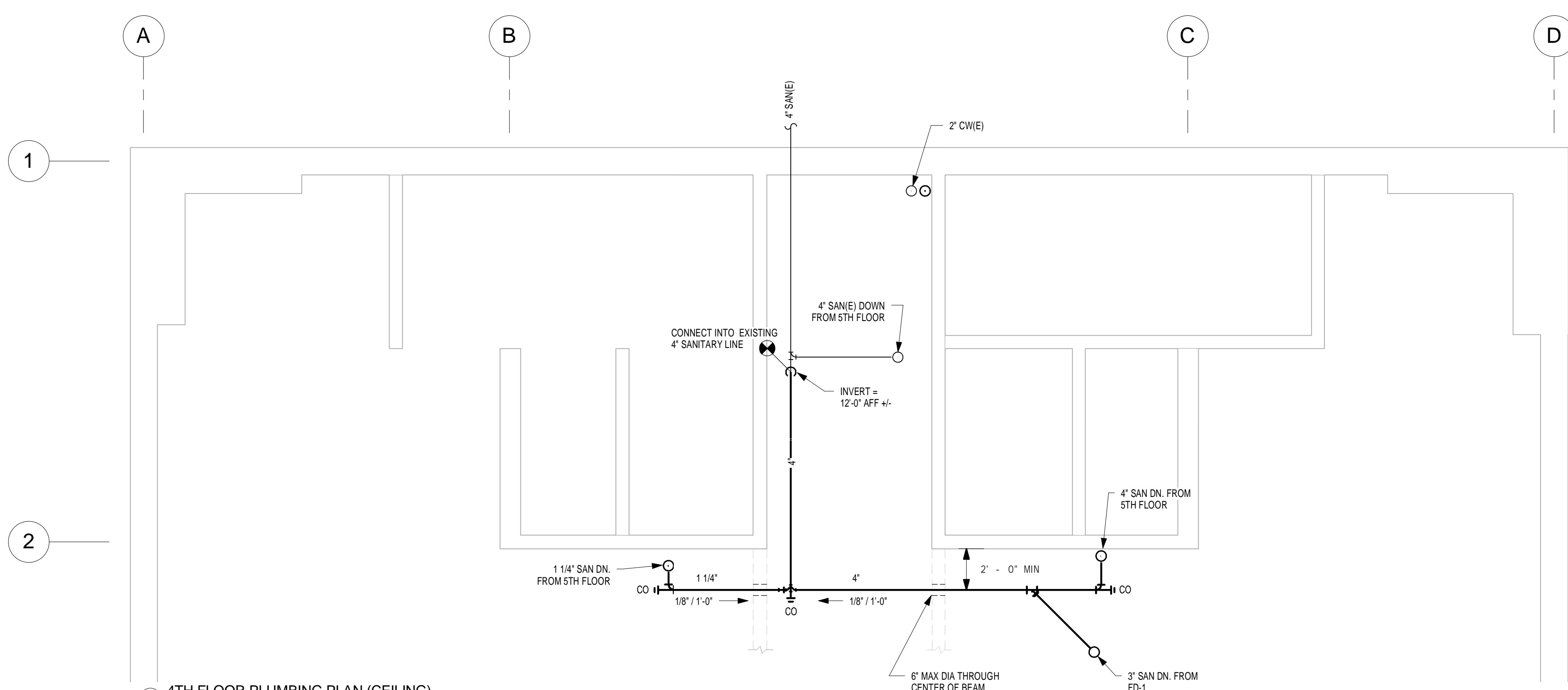
2 4TH FLOOR PLUMBING PLAN (CEILING) 1/4" = 1'-0"
